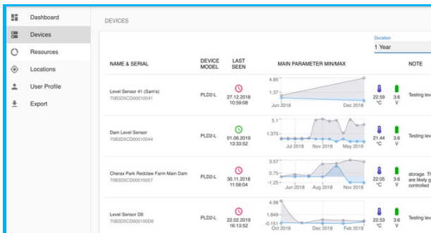
Single shot data visualization of devices
